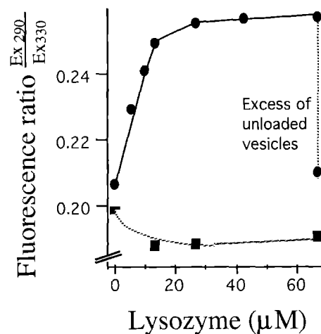
Fig. 2. The dependence of monomer fluorescence ratio at two excitation wavelengths (290 nm/330 nm) of dipyrène lipids on the lysozyme concentration. The vesicles consisted of DOPC/brain-PS/dipyr 10 PS (3:1:1) (●) and DOPC/dipyr 10 PC (4:1) (■). The total lipid concentration was kept constant to 10 \mu\text{M} during the protein titration. After addition of an excess of DOPC/brain-PS without pyrene lipid (final concentration 100 \mu\text{M} ) the ratio of monomeric pyrene fluorescence reverses to its initial value, indicating that the binding is reversible
