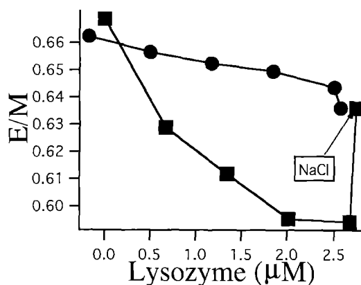
Fig. 7. The dependence of the excimer-monomer fluorescence intensity ratio (E/M) of dipyr 10 PS and dipyr 10 PC on the concentration of lysozyme. The total lipid concentration was kept constant (10 μM). Points ● show the effect on neutral PC/dipyr 10 PC (100:1) vesicles and points ■ that of DOPC/brain-PS/dipyr 10 PS (75:25:1) membranes. In the latter case, reversibility of this acyl chain effect is demonstrated by addition of an excess of NaCl to a final concentration of 100 mM
